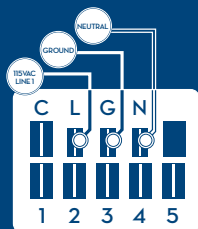
115VAC MOTOR
