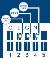
460VAC MOTOR
